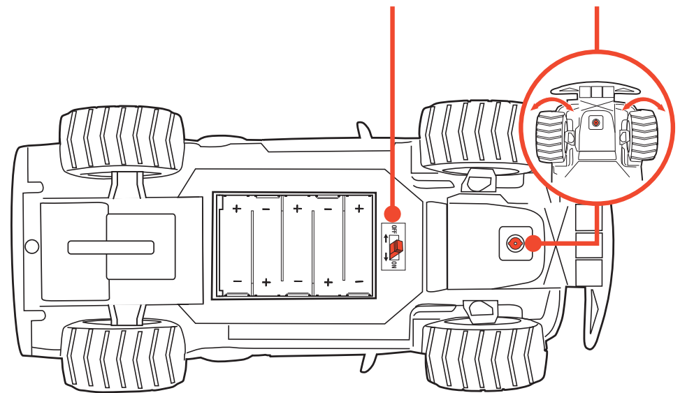
ON/OFF Switch
