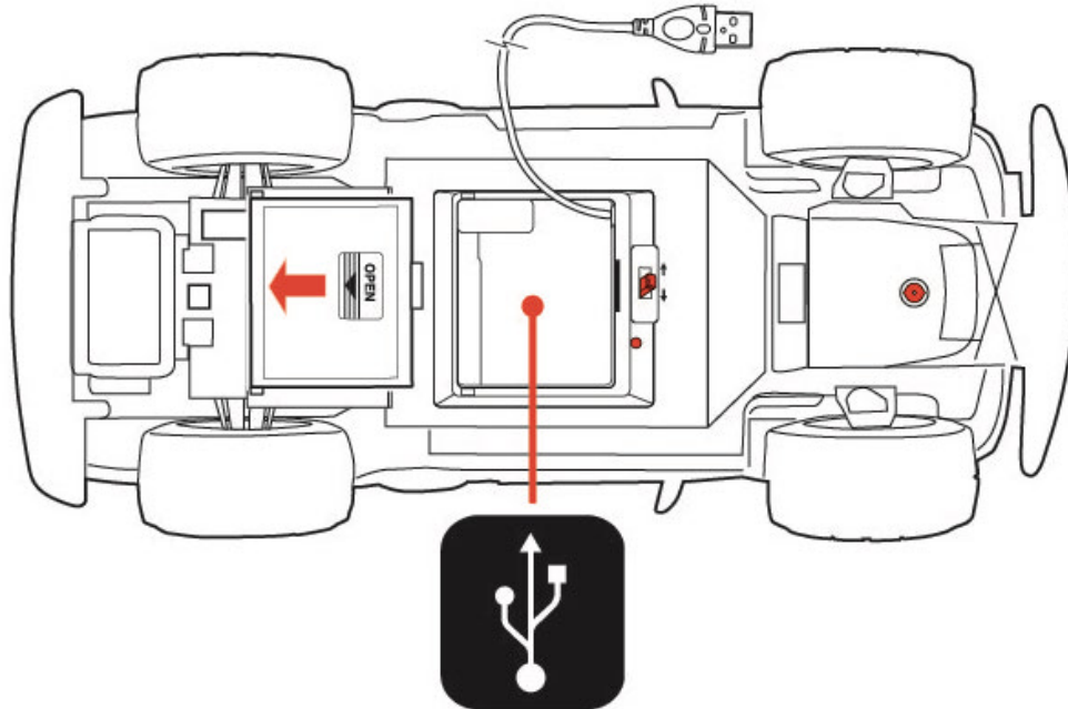
USB Charging Cable and Storage Compartment
